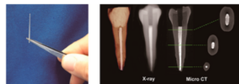
Nanodiamond-Gutta Percha Biomaterials for Root Canal Therapy
